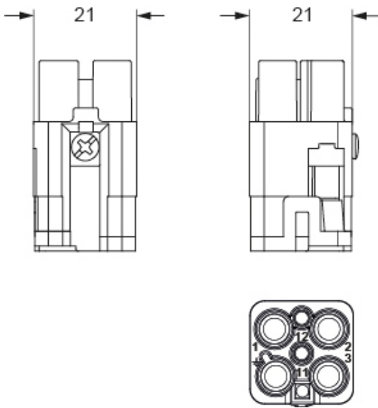
Catalogue drawings
