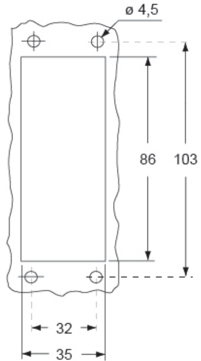
Catalogue drawings
