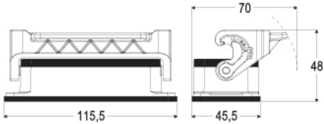
Catalogue drawings
