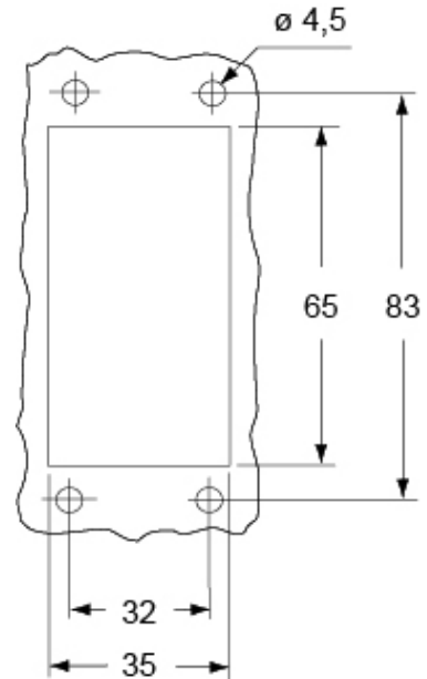
Catalogue drawings
