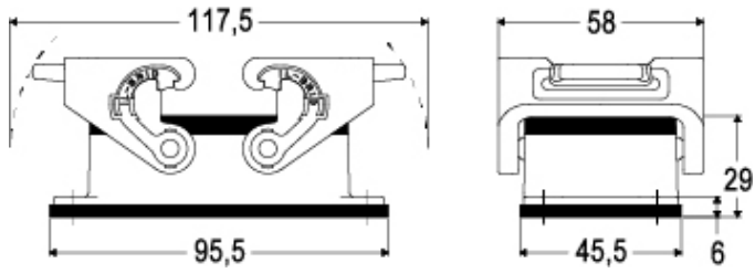
Catalogue drawings
