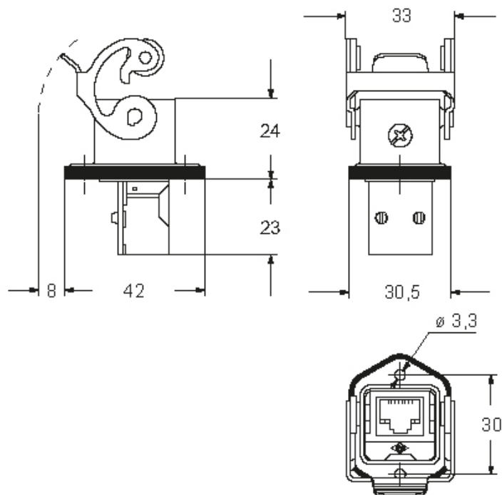
Catalogue drawings
