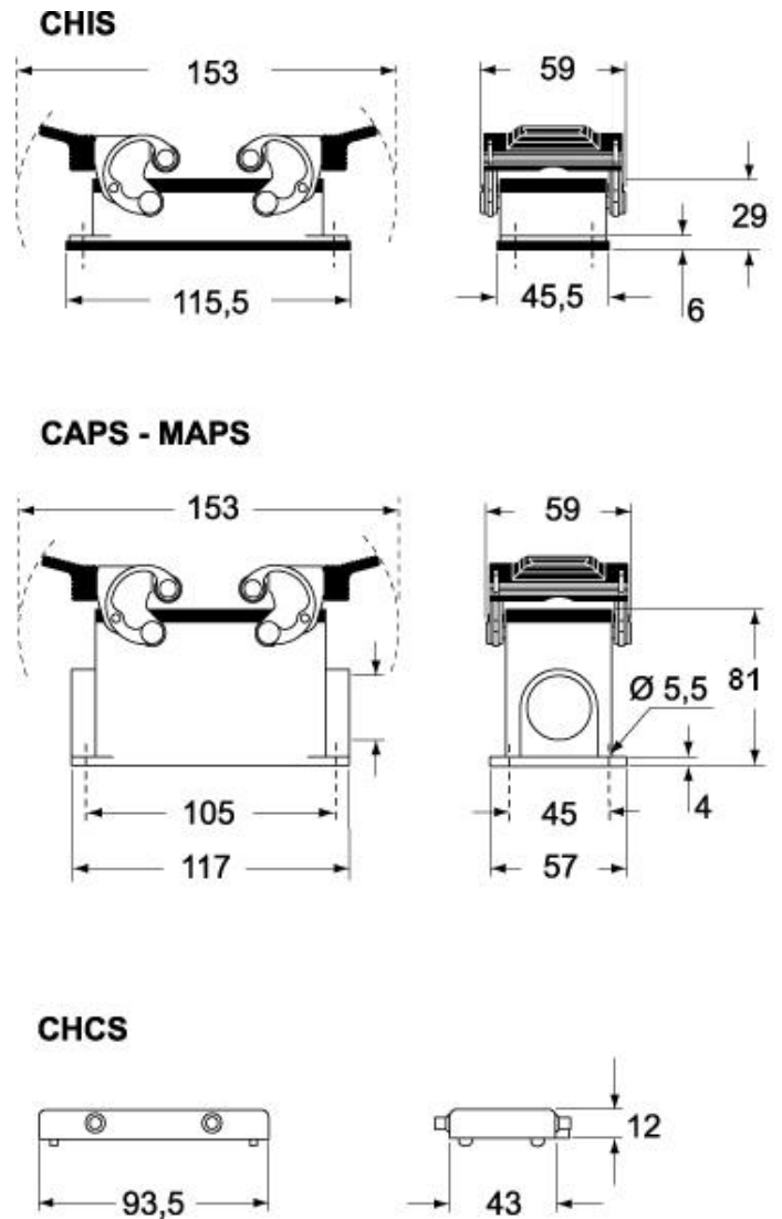
Catalogue drawings
