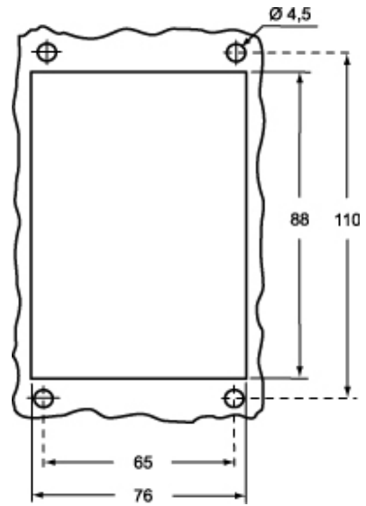
Catalogue drawings
