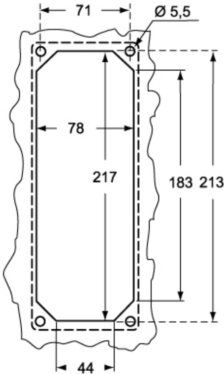
Catalogue drawings
