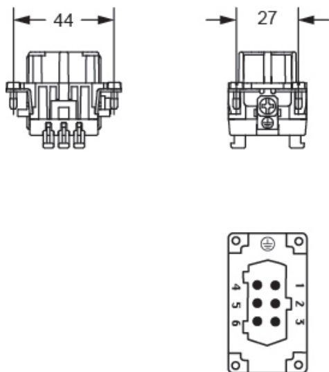
Catalogue drawings
