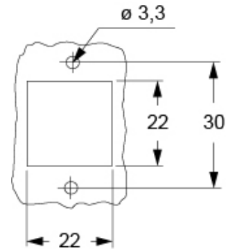
Catalogue drawings
