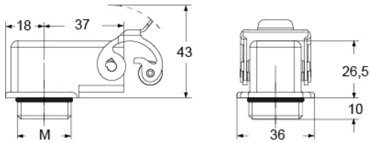
Catalogue drawings
