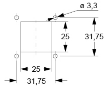
Catalogue drawings
