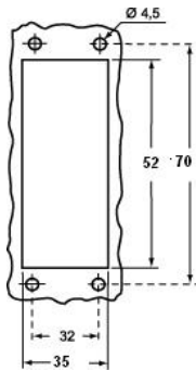
Catalogue drawings
