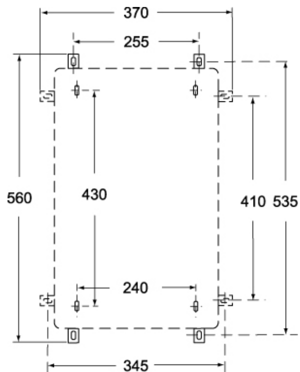
Catalogue drawings
