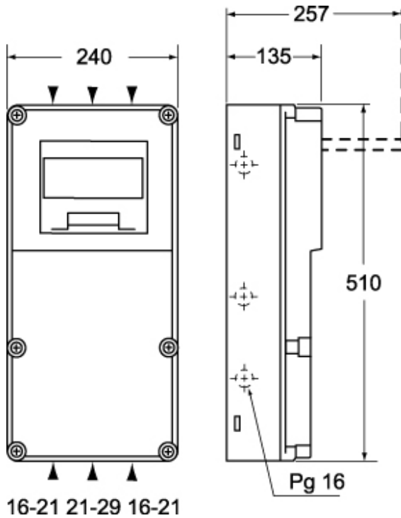
Catalogue drawings
