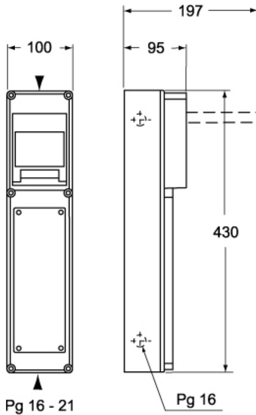
Catalogue drawings
