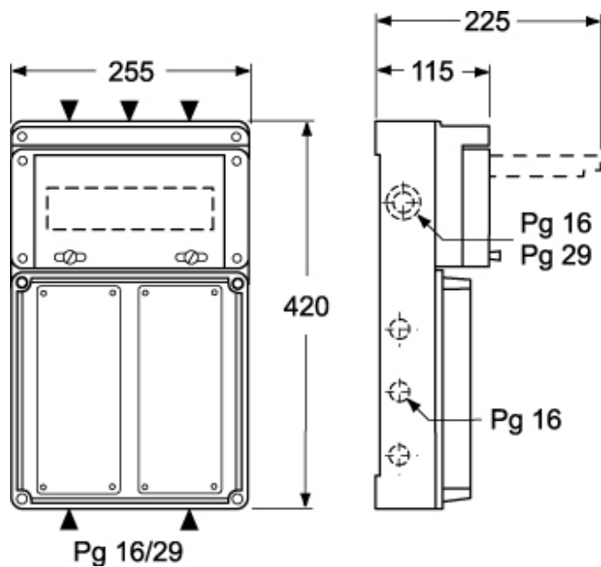
Catalogue drawings
