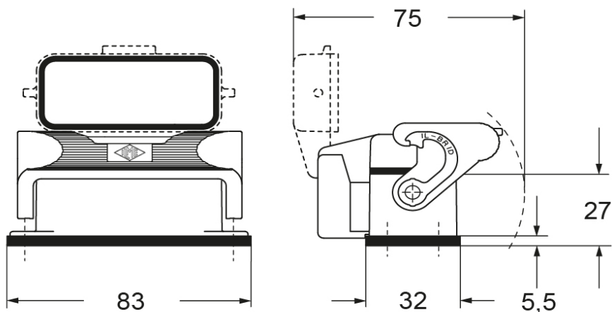
Catalogue drawings
