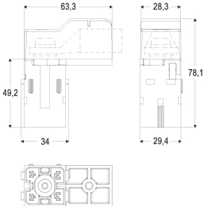
Catalogue drawings
