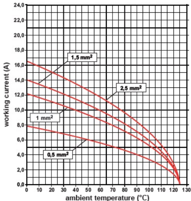
Derating curves
