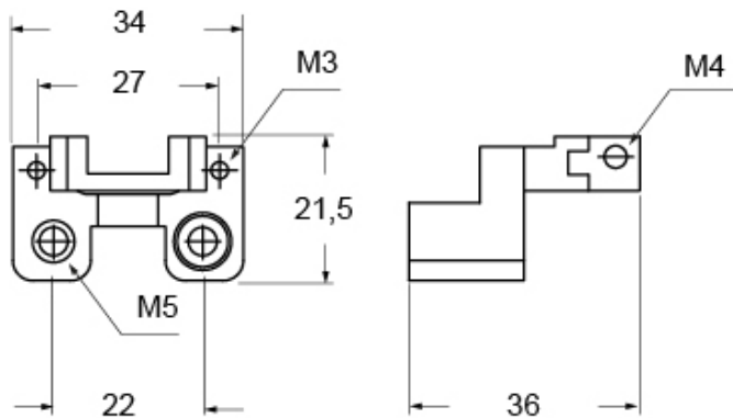
Catalogue drawings
