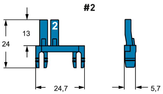
Catalogue drawings
