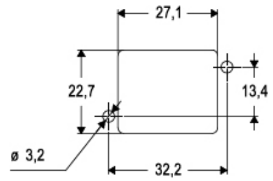
Catalogue drawings
