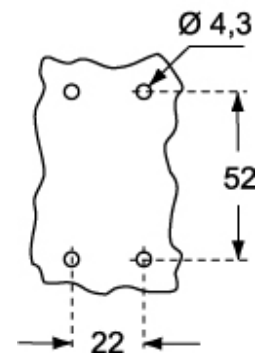
Catalogue drawings
