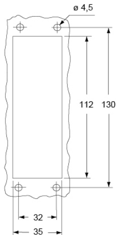
Catalogue drawings
