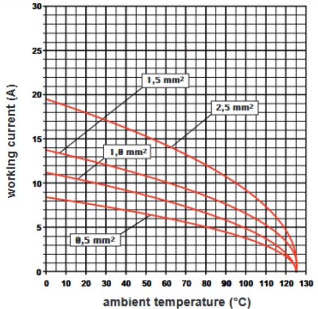
RDSH 27 poles connector inserts Maximum current load derating diagram
