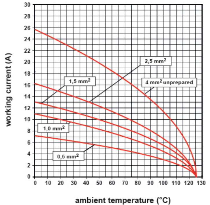
CQEY 32 poles connector inserts Maximum current load derating diagram
