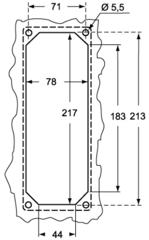
Catalogue drawings
