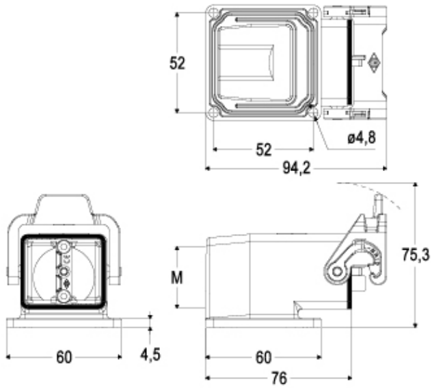
Catalogue drawings
