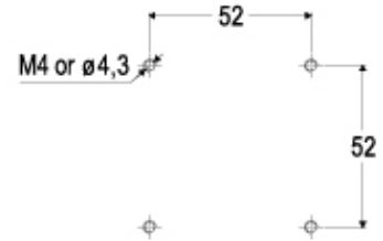
Catalogue drawings
