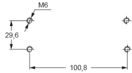
Catalogue drawings
