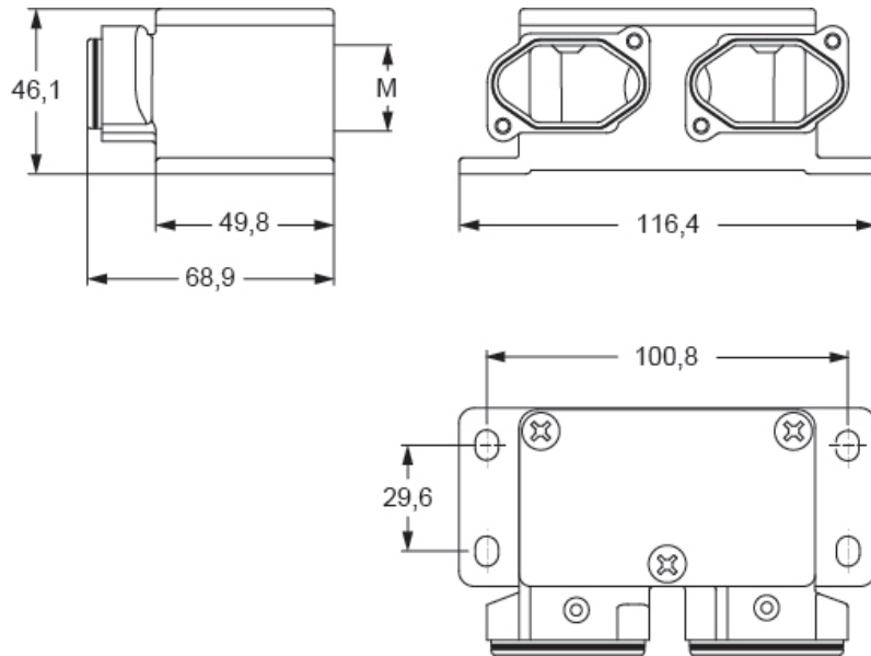
Catalogue drawings
