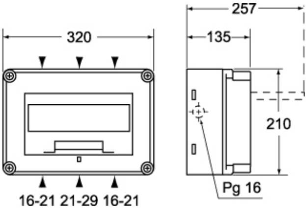
Catalogue drawings
