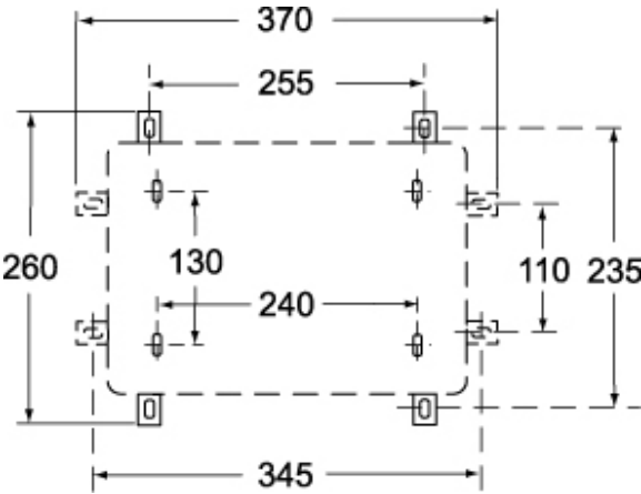
Catalogue drawings
