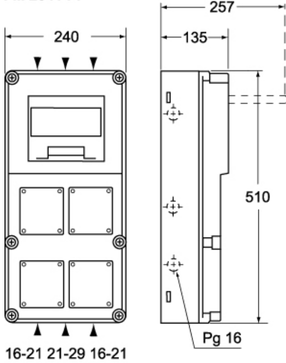
Catalogue drawings
