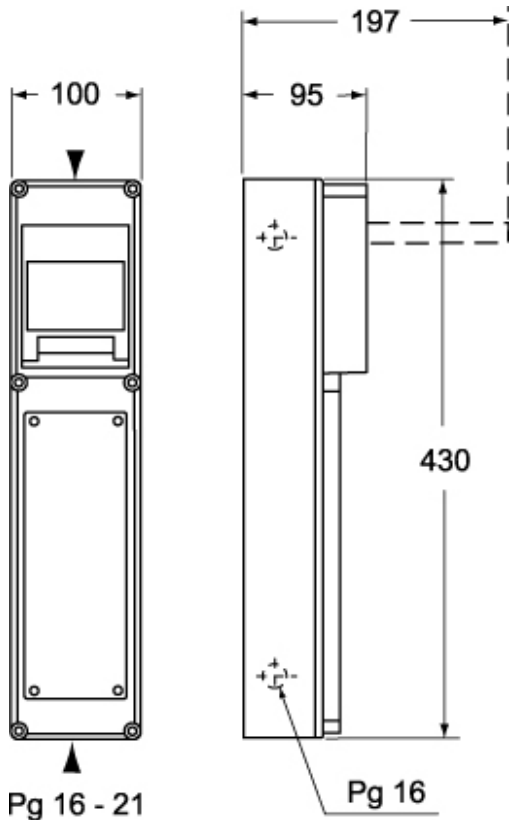
Catalogue drawings
