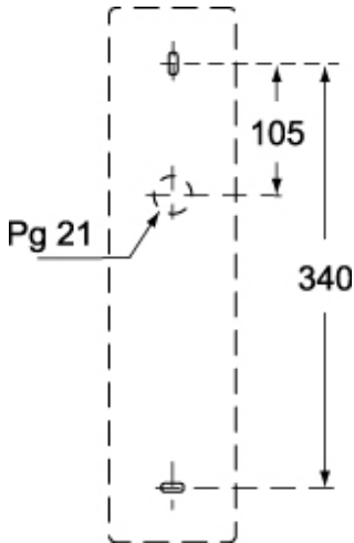
Catalogue drawings
