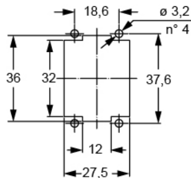
Catalogue drawings
