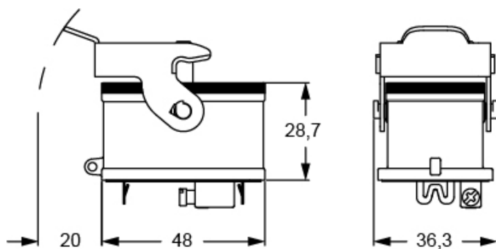
Catalogue drawings
