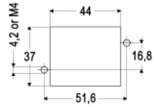
Catalogue drawings
