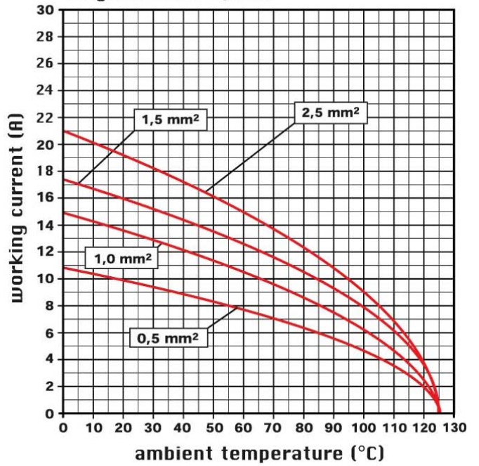
diagram CSH 32 poles
