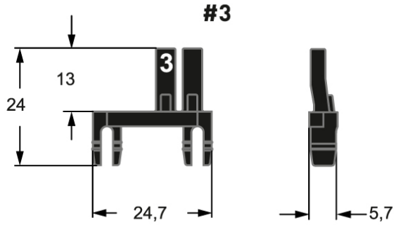
Catalogue drawings
