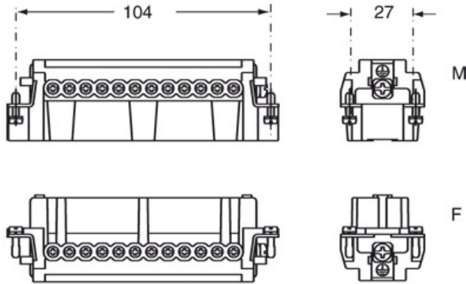
Catalogue drawings
