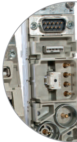
MIXO COAX, RJ45, USB, D-Sub, Contacts for high voltage and coaxial cables
