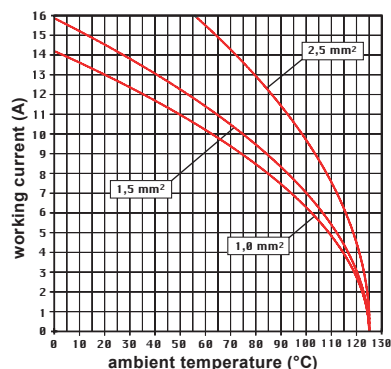
CDY 07 inserts maximum current load derating diagram
