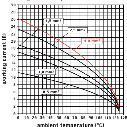
diagram CCE 10 poles
