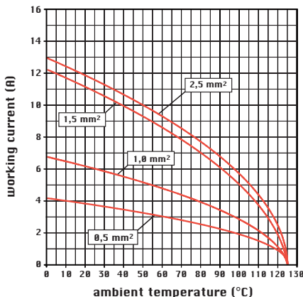
diagram CDD 42 poles
