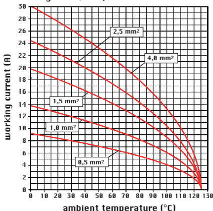
diagram CQE 10 poles
