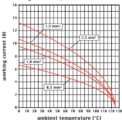
diagram CDD 38 poles
