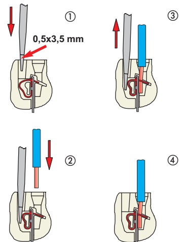
Connection with spring terminal
