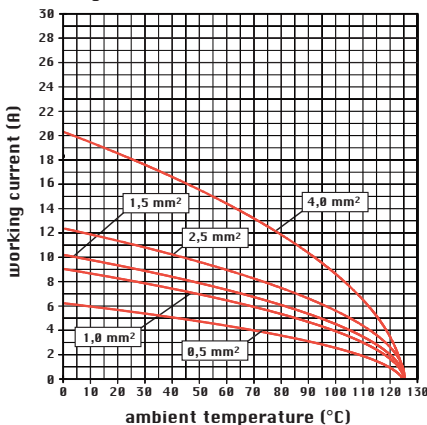
diagram CQE 92 poles
