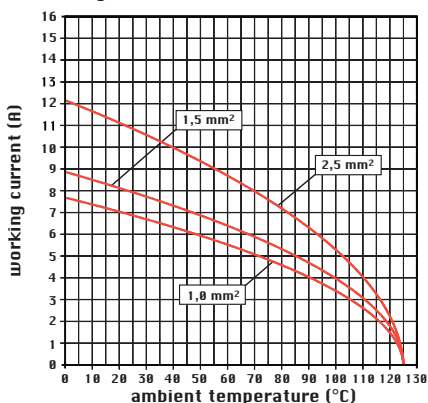
diagram CD 40 poles
