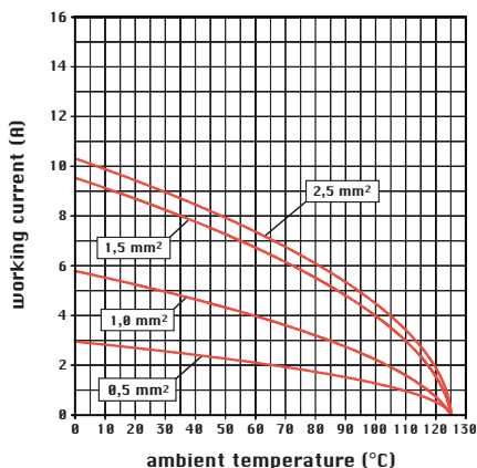
diagram CDD 216 poles
