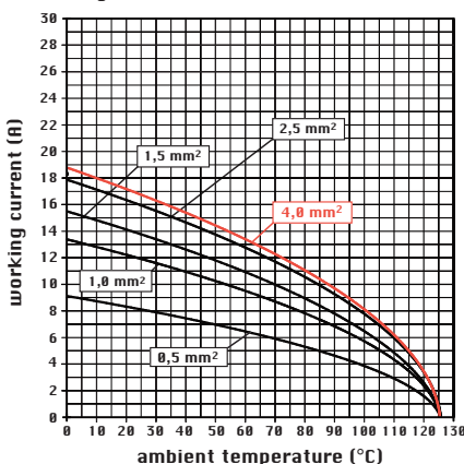
diagram CCE 24 poles
