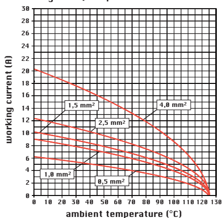
diagram CQE 46 poles
